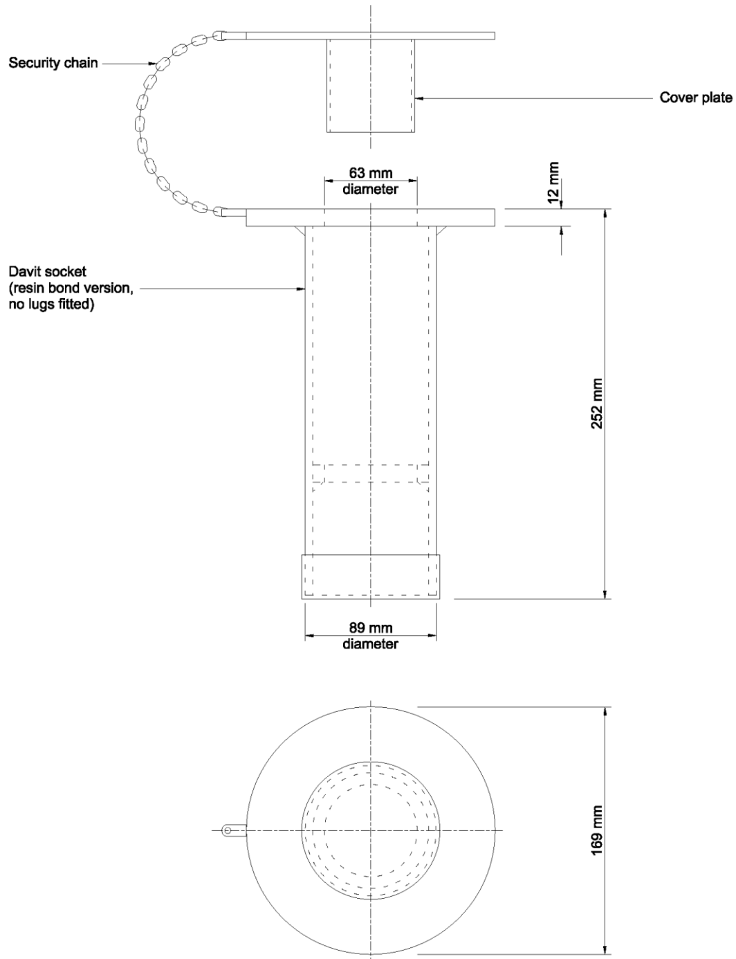
Figure D 1 Standard flush mount davit socket
