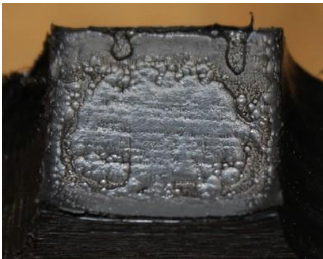
Plate A.2: Mixed mode failure
