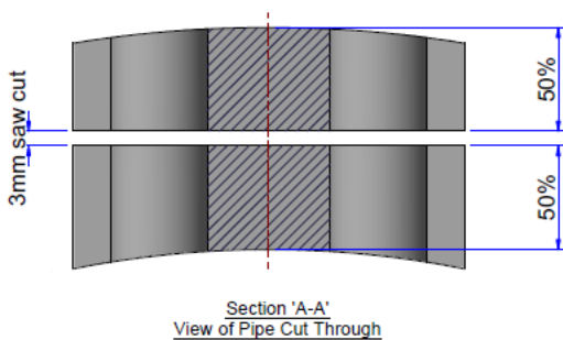
Figure 5 Preparation of samples from thick walled pipes
