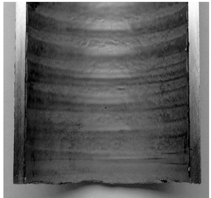
Figure 6 - Ridged lining
