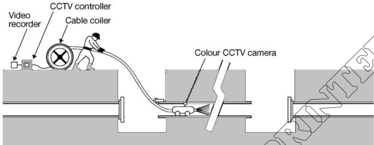
Figure 3 – CCTV inspection
