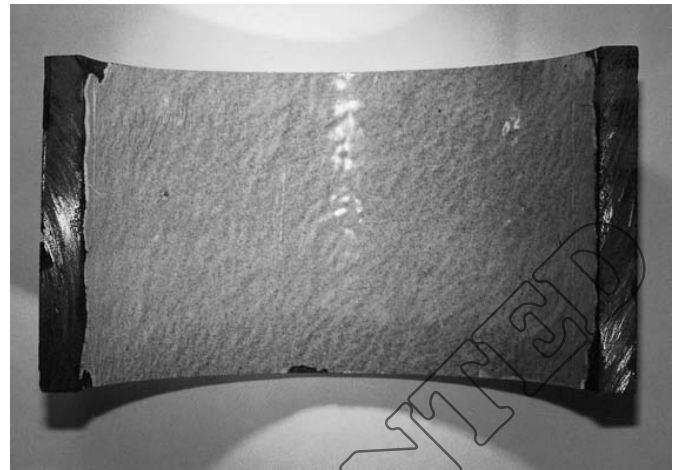
Figure 18 – Speckled lining
