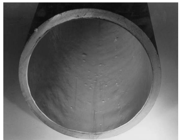
Figure 17 – 'Blowholes' in lining
